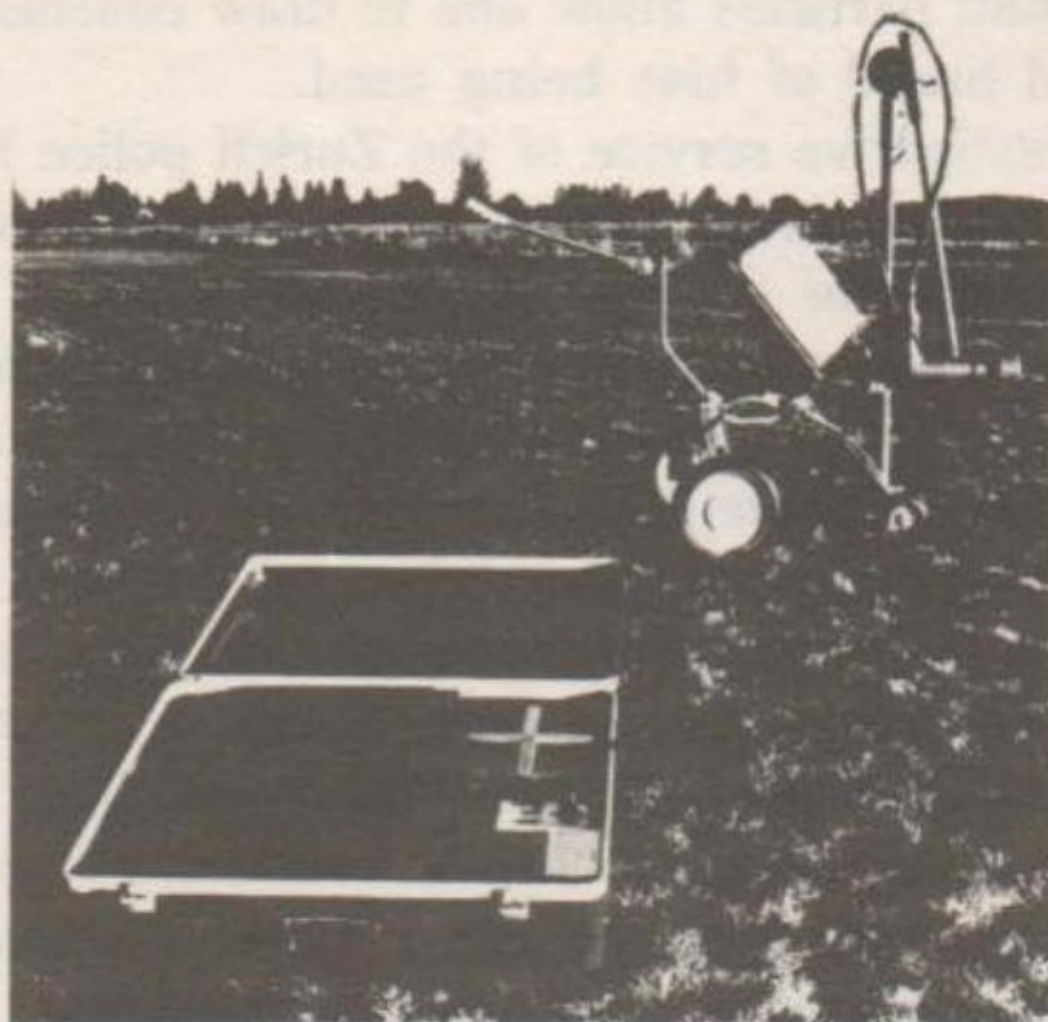
Portable x-ray equipment used in investigating the sites of explosives crimes.
