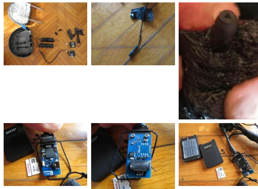
1: control unit; 2: batteries; 3: GPS antenna; 4: microphone; 5: SIM card 2: two batteries of the listening device; 4: microphones connected to the listening device; 6: dismantled listening device; 7: SD card
