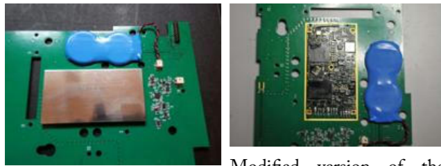
Modified version of the phone largest circuit board (with surveillance device). The battery pack (in blue) and the shielded module (in light brown) are part of the surveillance device.
